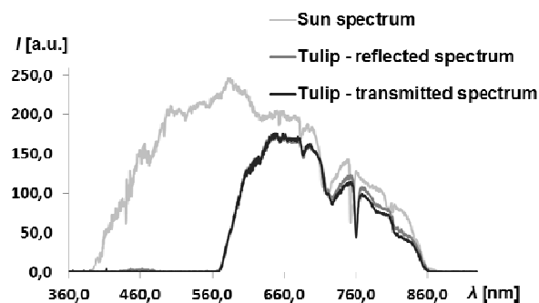
Figure 6. The transmitted and reflected spectrum of the tulip flower compared with the sun spectrum
