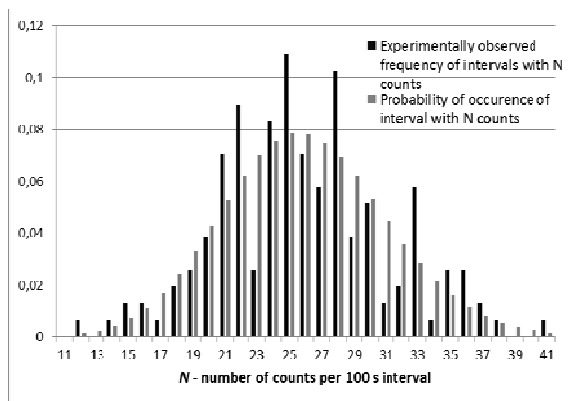
Figure 3. Poisson distribution
