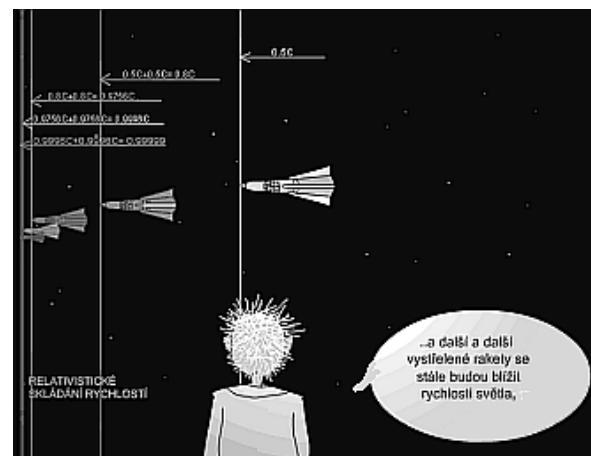
Figure 3. Adding velocities
