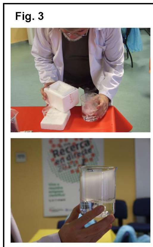
Fig. 3. Sublimation of dry ice.
